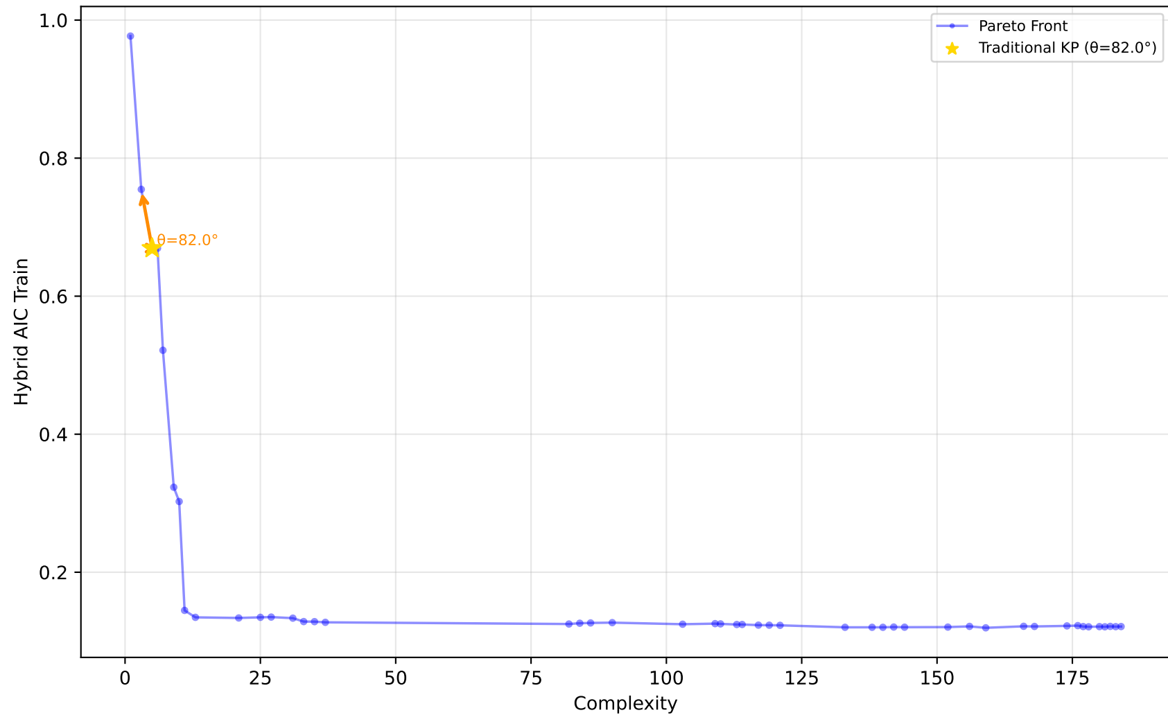
529_pollen - Run 18 - SVP - Hybrid AIC Train \lambda_1=0.60, \lambda_2=0.40, \lambda_3=1.00 | Difficulty: 1.00 | Method: hmr
