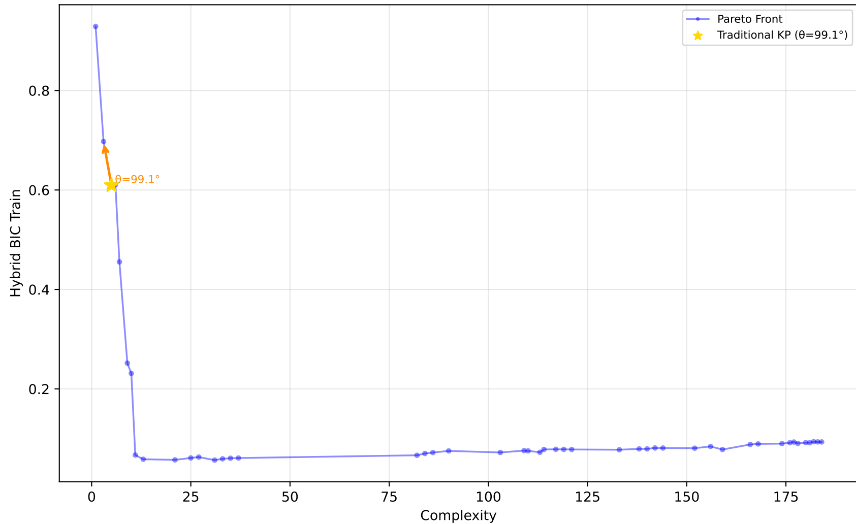
529_pollen - Run 18 - SVP - Hybrid BIC Train \lambda_1=0.10, \lambda_2=0.80, \lambda_3=0.30 | Difficulty: 1.00 | Method: hmr
