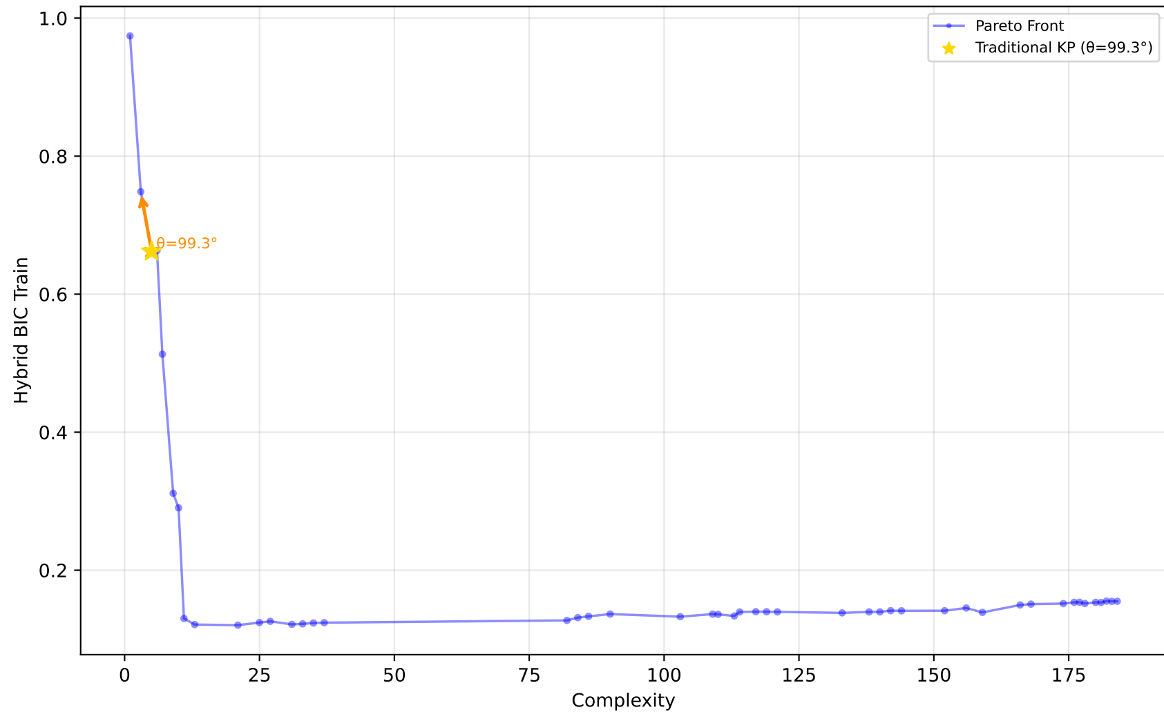
529_pollen - Run 18 - SVP - Hybrid BIC Train \lambda_1=0.60, \lambda_2=0.40, \lambda_3=1.00 | Difficulty: 1.00 | Method: hmr
