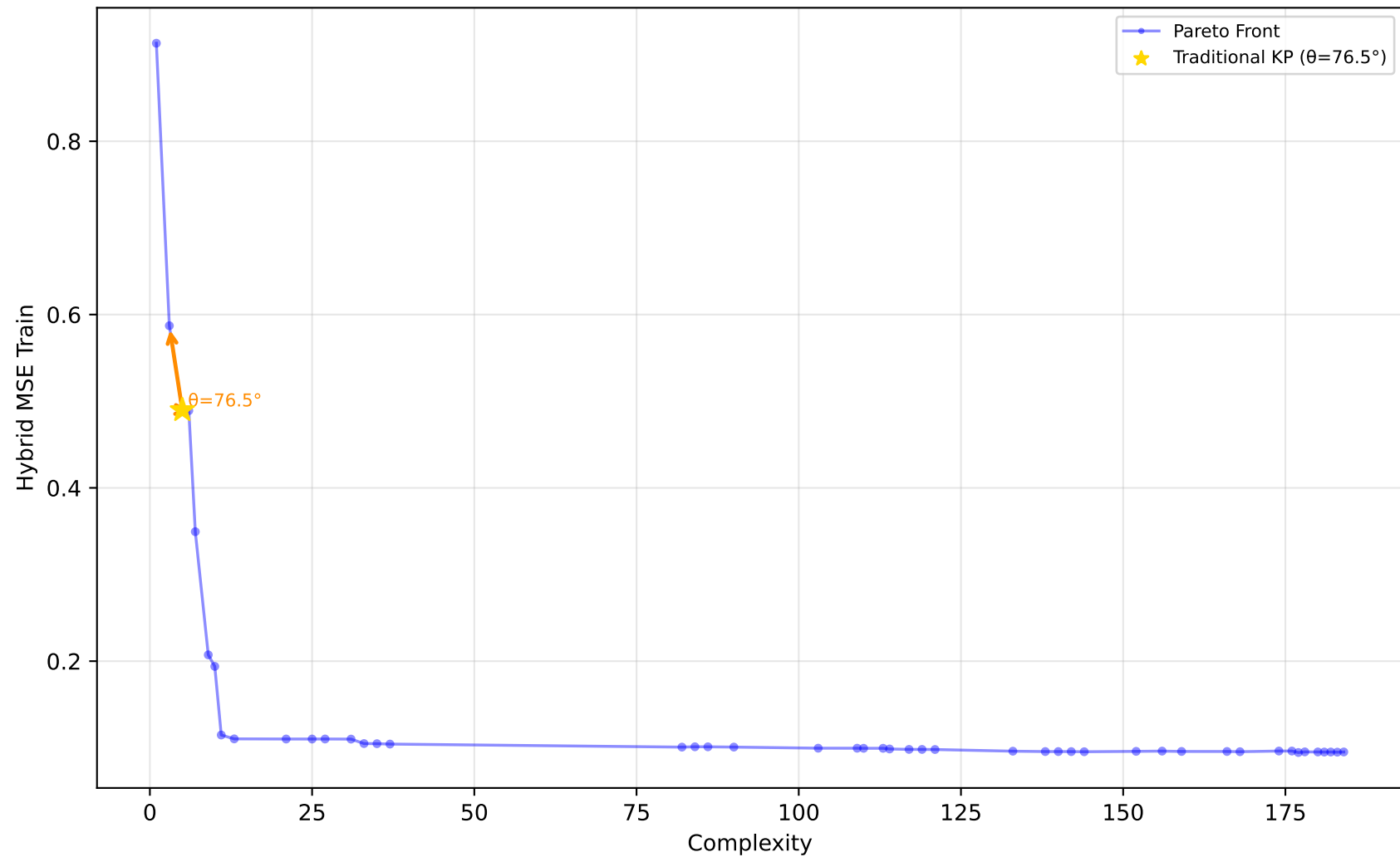
529_pollen - Run 18 - SVP - Hybrid MSE Train \lambda_1=0.60, \lambda_2=0.40, \lambda_3=1.00 | Difficulty: 1.00 | Method: hmr
