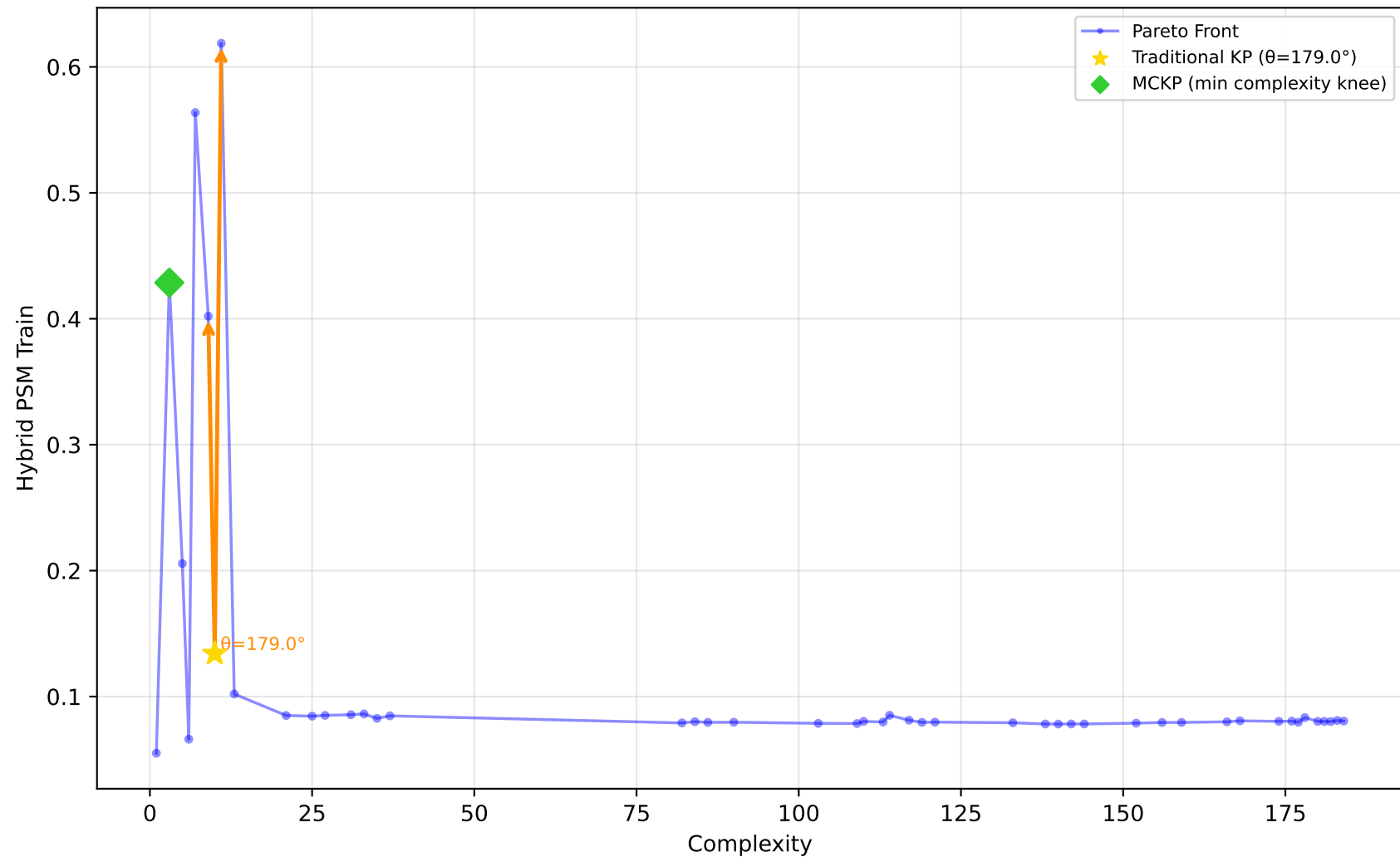
529_pollen - Run 18 - SVP - Hybrid PSM Train \lambda_1=0.60, \lambda_2=0.40, \lambda_3=1.00 | Difficulty: 1.00 | Method: hmr
