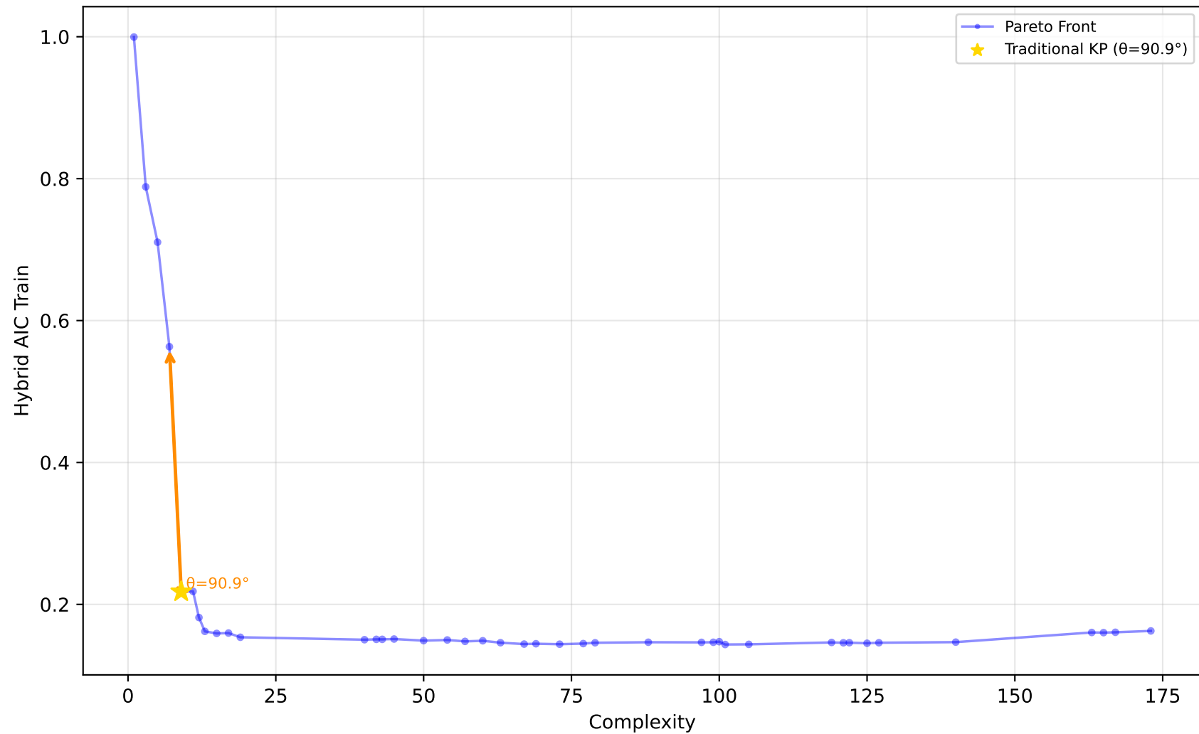
529_pollen - Run 19 - MVP - Hybrid AIC Train \lambda_1=0.90, \lambda_2=0.00, \lambda_3=0.00 | Difficulty: 1.00 | Method: hmr
