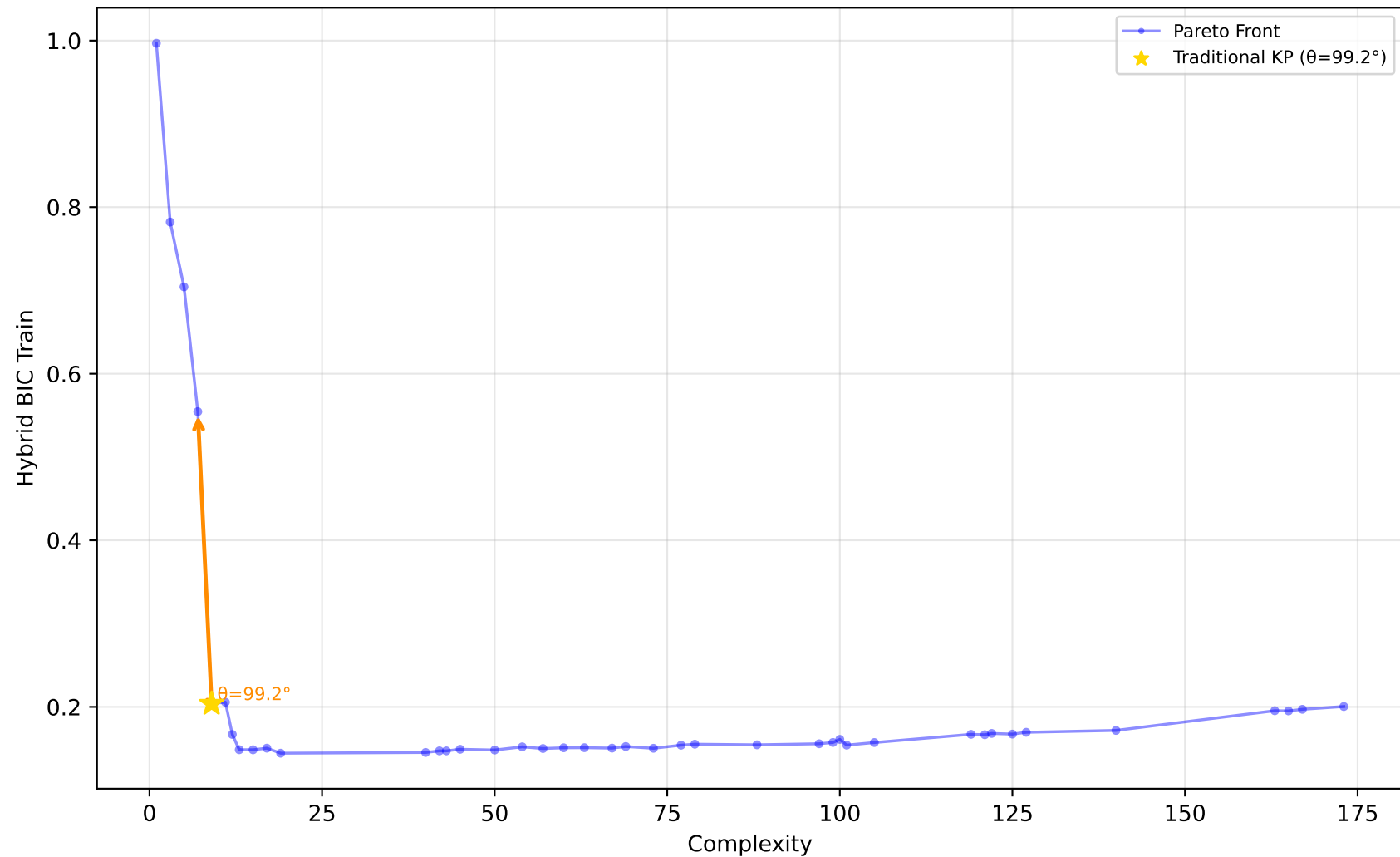
529_pollen - Run 19 - MVP - Hybrid BIC Train \lambda_1=0.90, \lambda_2=0.00, \lambda_3=0.00 | Difficulty: 1.00 | Method: hmr
