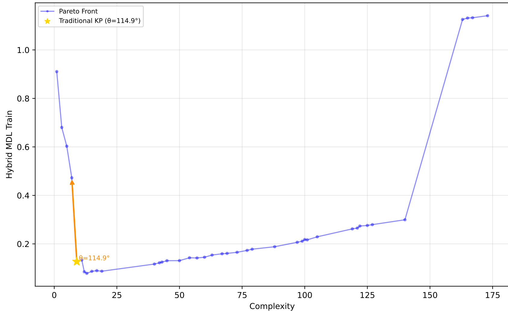
529_pollen - Run 19 - MVP - Hybrid MDL Train \lambda_1=0.00, \lambda_2=1.00, \lambda_3=0.80 | Difficulty: 1.00 | Method: hmr
