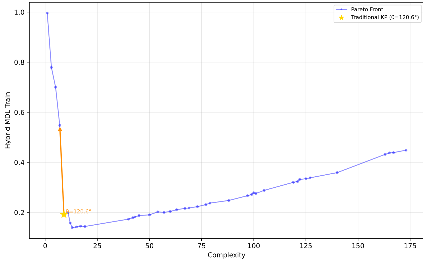
529_pollen - Run 19 - MVP - Hybrid MDL Train \lambda_1=0.90, \lambda_2=0.00, \lambda_3=0.00 | Difficulty: 1.00 | Method: hmr
