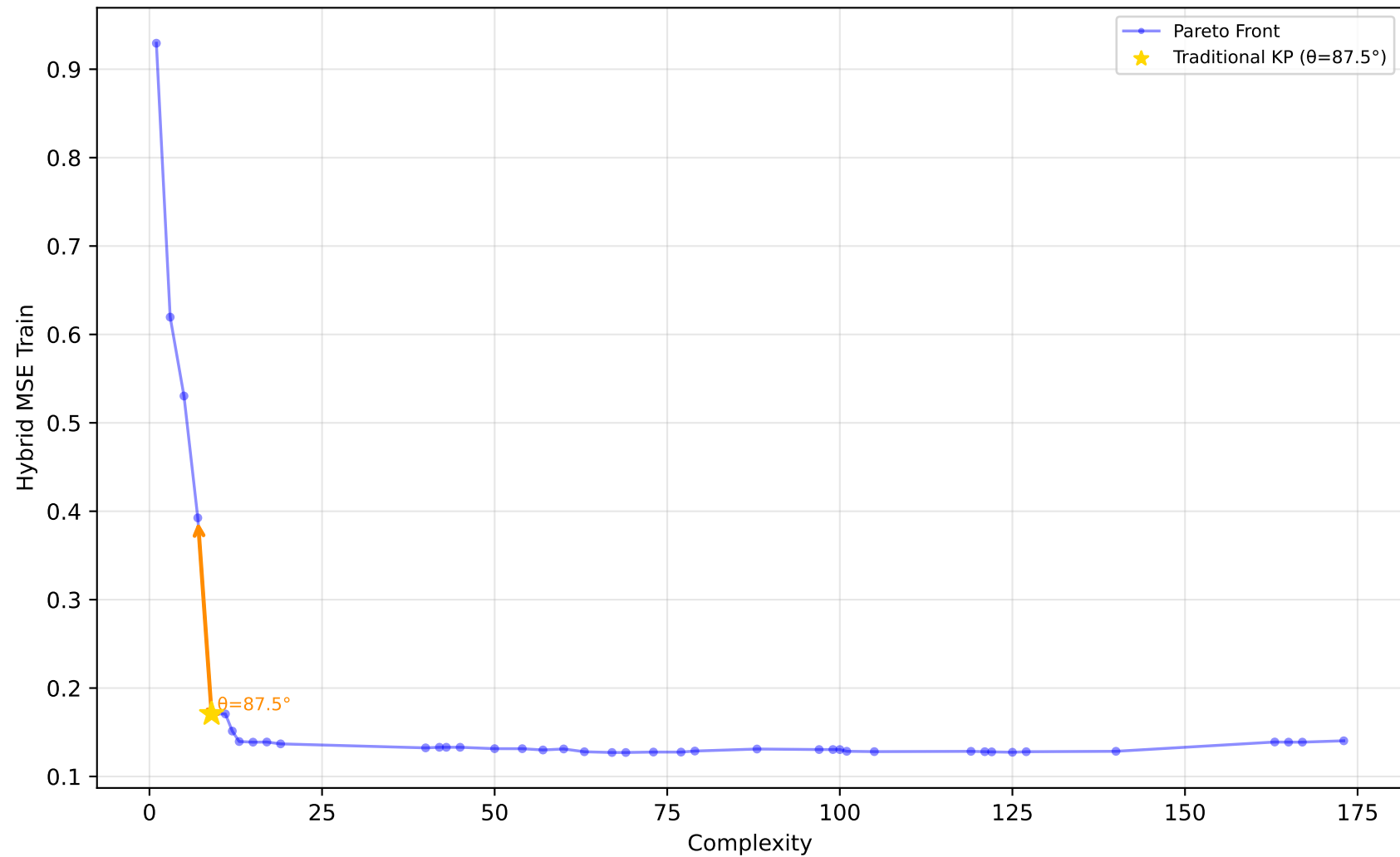
529_pollen - Run 19 - MVP - Hybrid MSE Train \lambda_1=0.90, \lambda_2=0.00, \lambda_3=0.00 | Difficulty: 1.00 | Method: hmr
