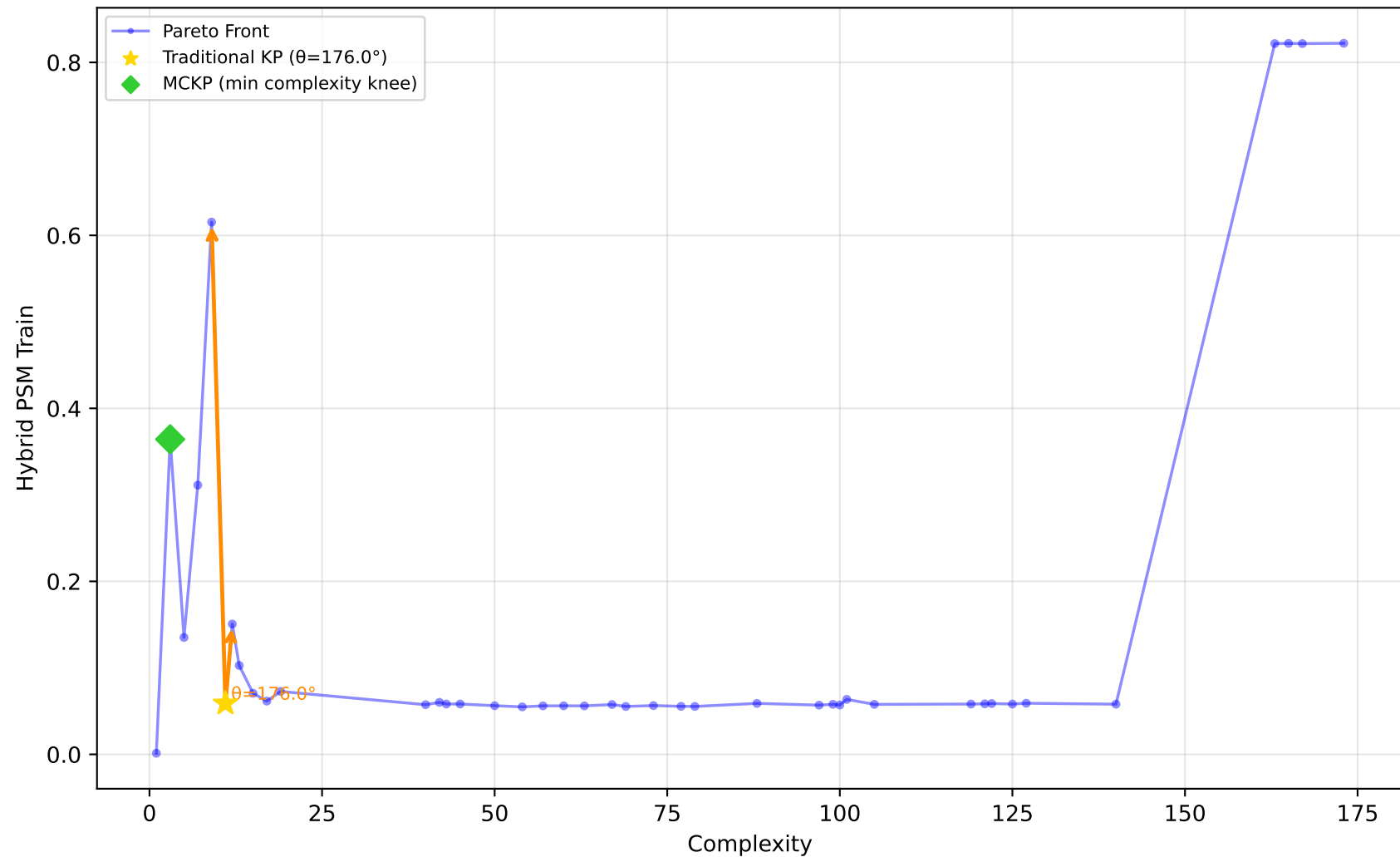
529_pollen - Run 19 - MVP - Hybrid PSM Train \lambda_1=0.00, \lambda_2=1.00, \lambda_3=0.80 | Difficulty: 1.00 | Method: hmr
