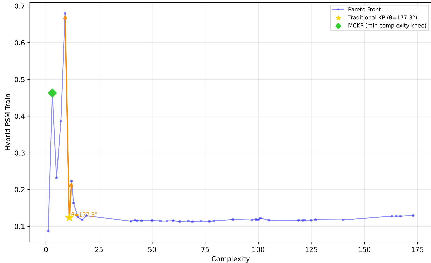
529_pollen - Run 19 - MVP - Hybrid PSM Train \lambda_1=0.90, \lambda_2=0.00, \lambda_3=0.00 | Difficulty: 1.00 | Method: hmr
