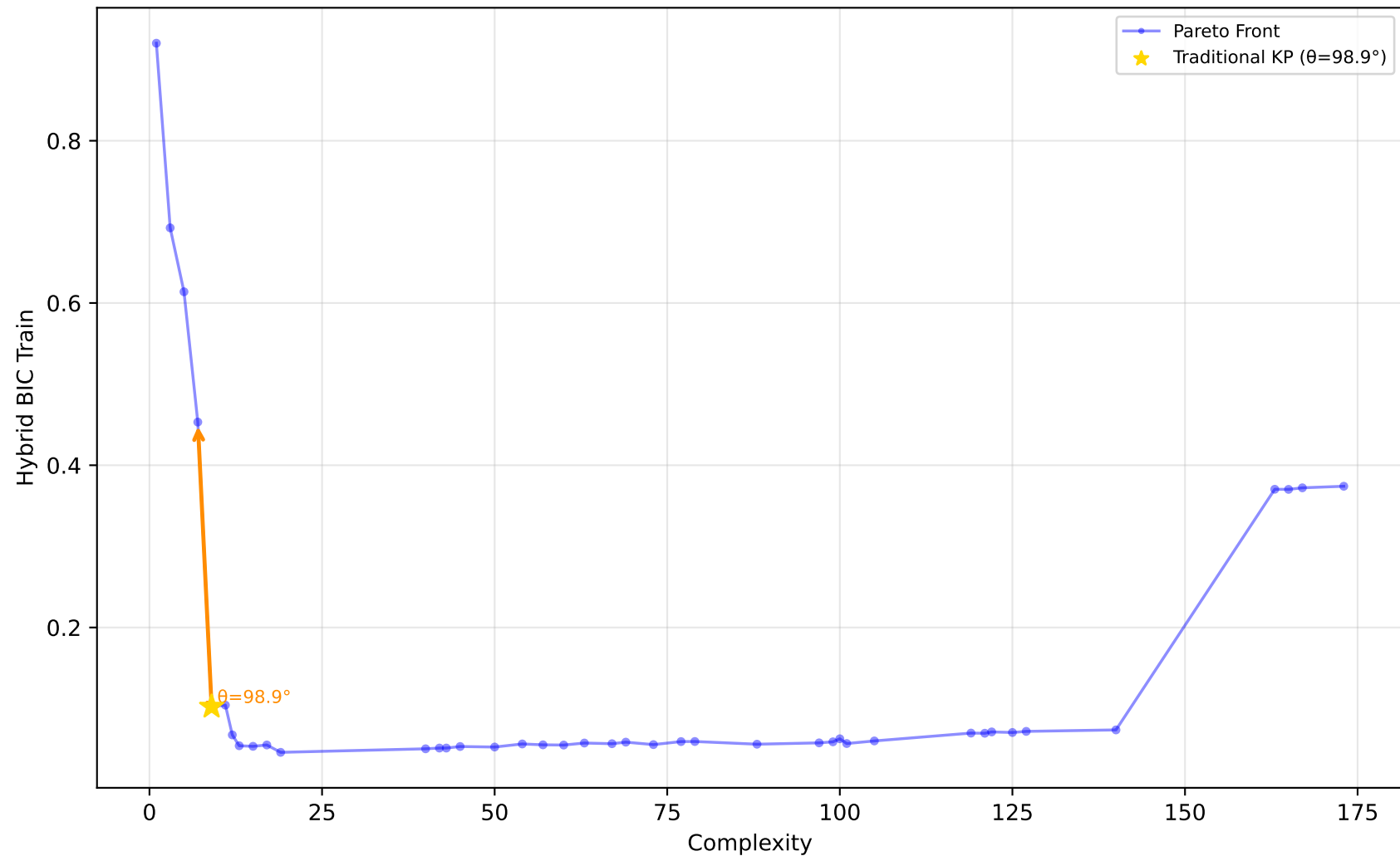
529_pollen - Run 19 - SVP - Hybrid BIC Train \lambda_1=0.10, \lambda_2=0.80, \lambda_3=0.30 | Difficulty: 1.00 | Method: hmr
