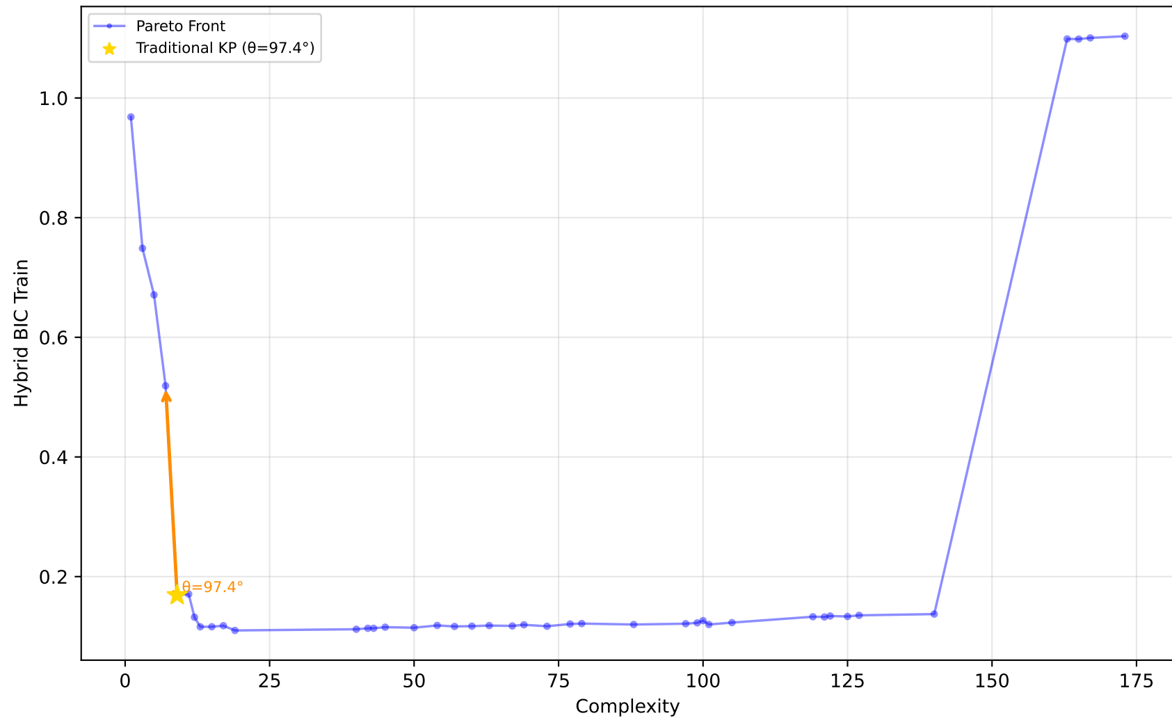
529_pollen - Run 19 - SVP - Hybrid BIC Train \lambda_1=0.60, \lambda_2=0.40, \lambda_3=1.00 | Difficulty: 1.00 | Method: hmr
