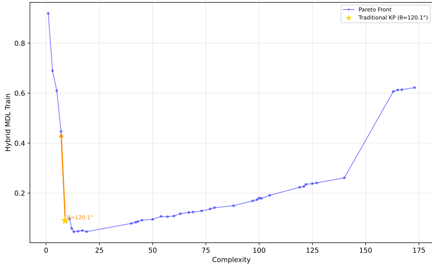
529_pollen - Run 19 - SVP - Hybrid MDL Train \lambda_1=0.10, \lambda_2=0.80, \lambda_3=0.30 | Difficulty: 1.00 | Method: hmr
