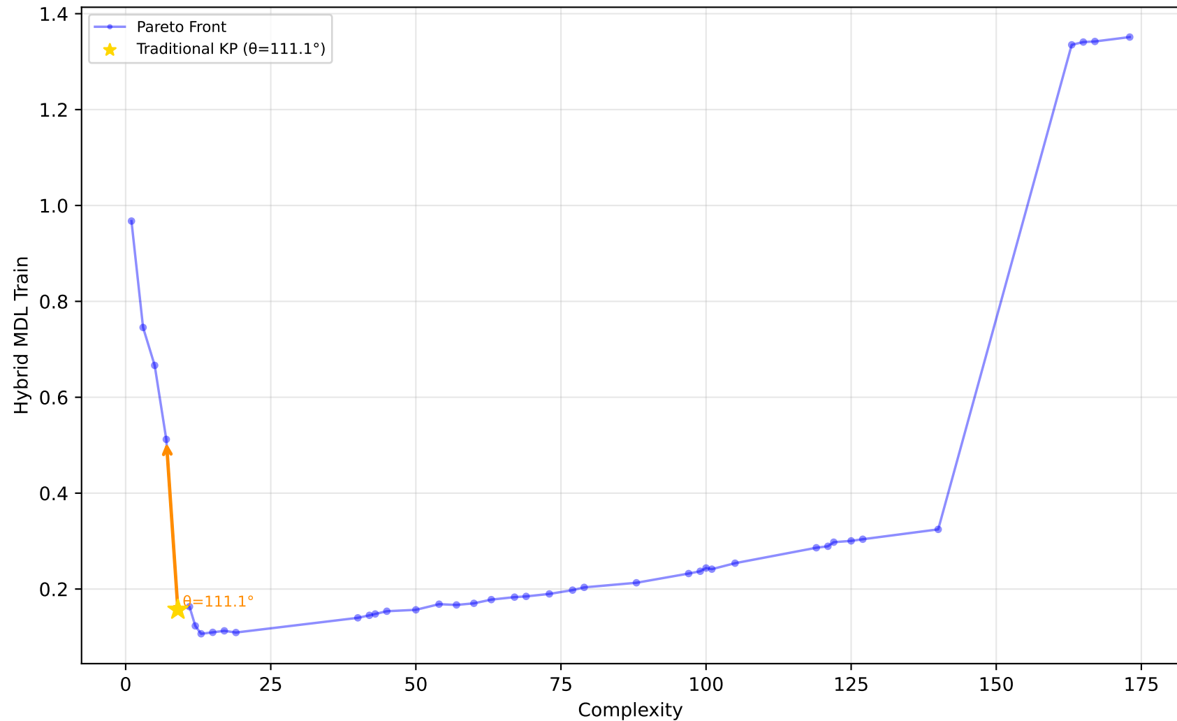
529_pollen - Run 19 - SVP - Hybrid MDL Train \lambda_1=0.60, \lambda_2=0.40, \lambda_3=1.00 | Difficulty: 1.00 | Method: hmr
