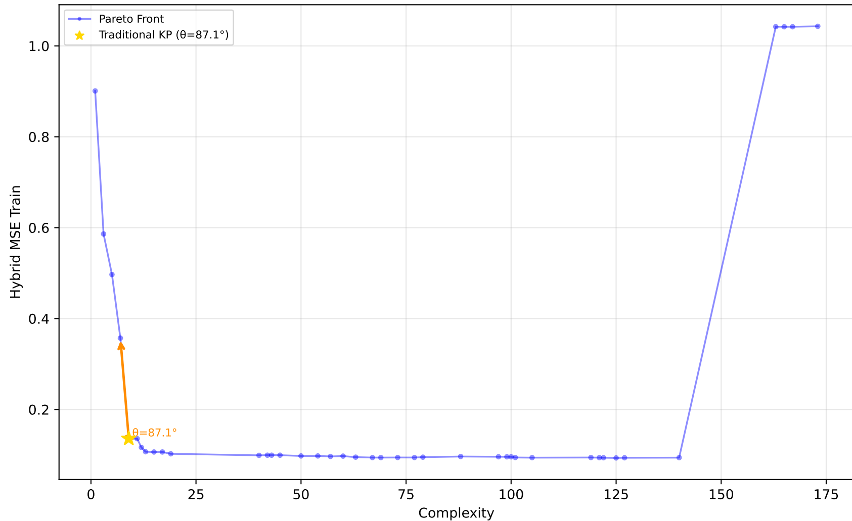
529_pollen - Run 19 - SVP - Hybrid MSE Train \lambda_1=0.60, \lambda_2=0.40, \lambda_3=1.00 | Difficulty: 1.00 | Method: hmr
