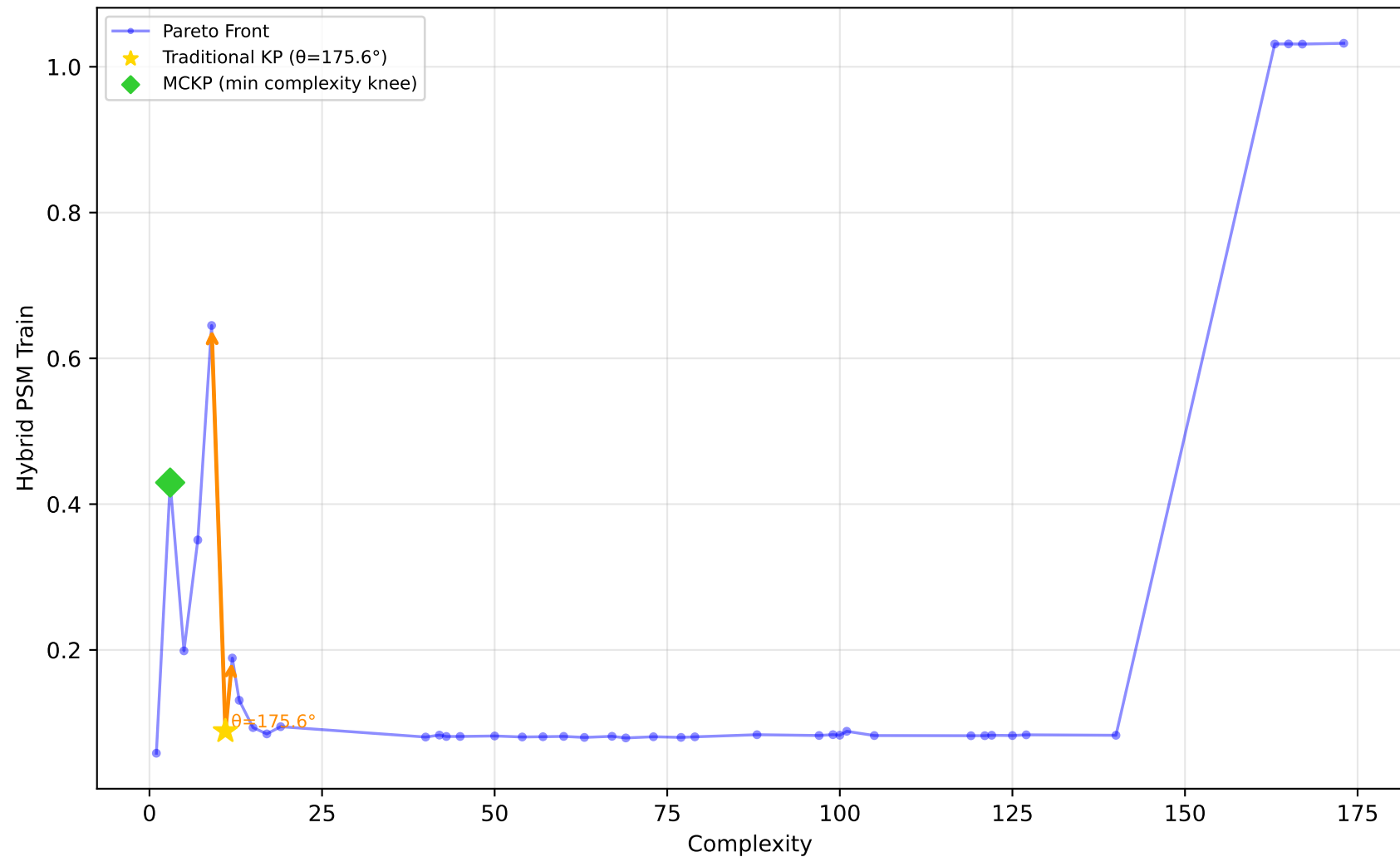
529_pollen - Run 19 - SVP - Hybrid PSM Train \lambda_1=0.60, \lambda_2=0.40, \lambda_3=1.00 | Difficulty: 1.00 | Method: hmr
