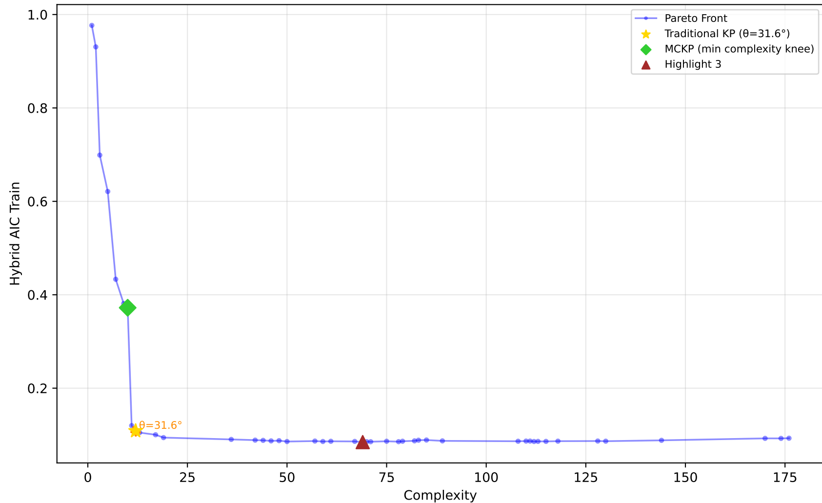
529_pollen - Run 1 - MVP - Hybrid AIC Train \lambda_1=0.00, \lambda_2=1.00, \lambda_3=0.80 | Difficulty: 1.00 | Method: hmr
