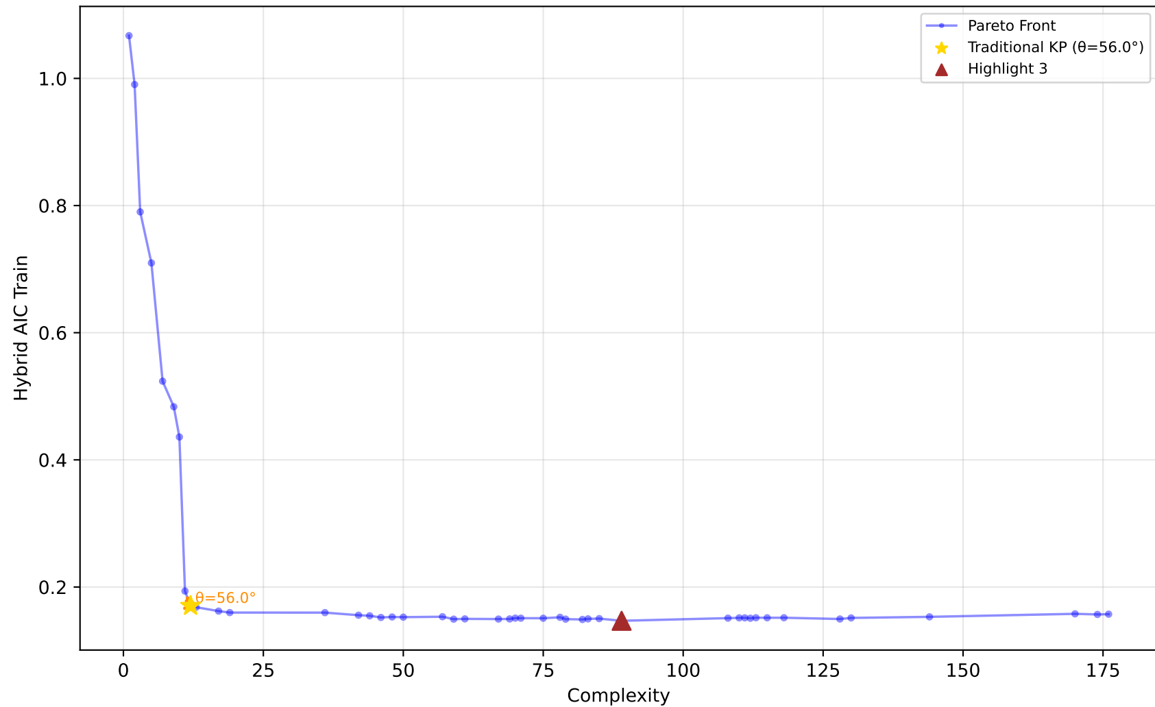
529_pollen - Run 1 - MVP - Hybrid AIC Train \lambda_1=0.90, \lambda_2=0.00, \lambda_3=0.00 | Difficulty: 1.00 | Method: hmr
