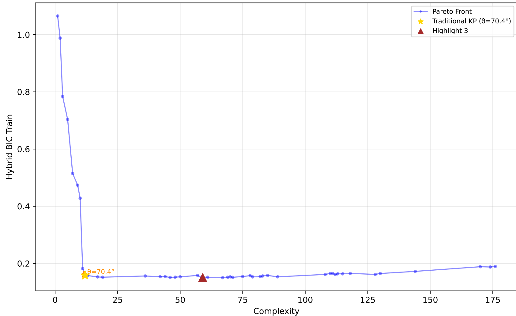
529_pollen - Run 1 - MVP - Hybrid BIC Train \lambda_1=0.90, \lambda_2=0.00, \lambda_3=0.00 | Difficulty: 1.00 | Method: hmr
