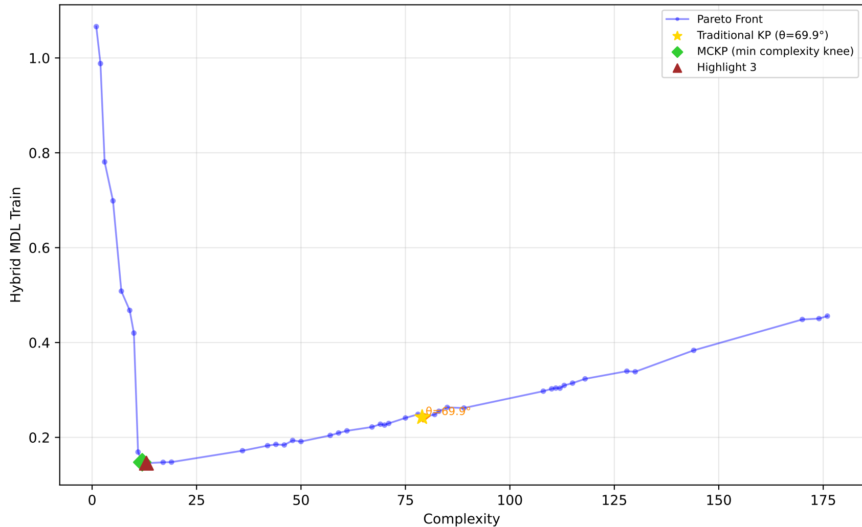
529_pollen - Run 1 - MVP - Hybrid MDL Train \lambda_1=0.90, \lambda_2=0.00, \lambda_3=0.00 | Difficulty: 1.00 | Method: hmr
