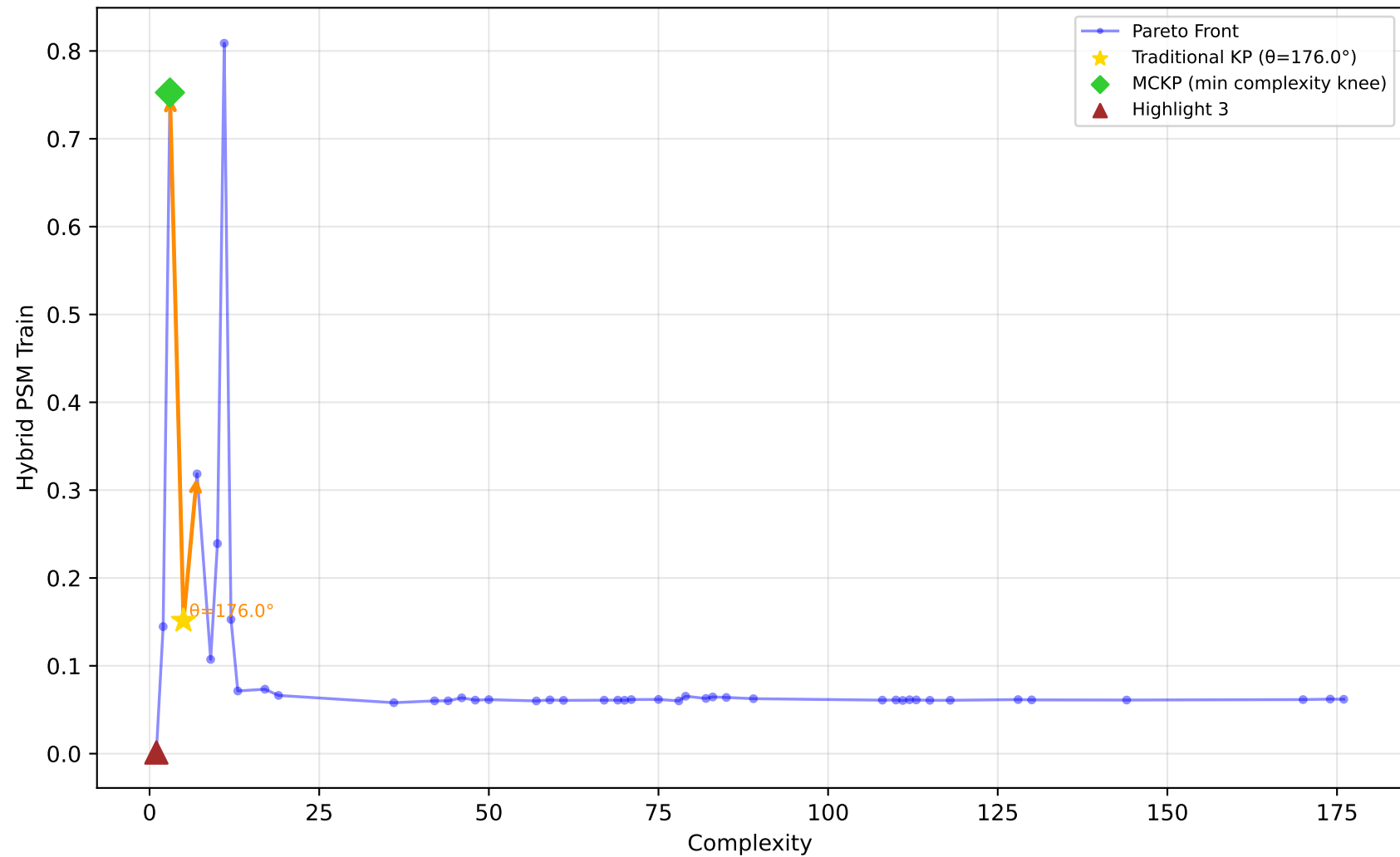
529_pollen - Run 1 - MVP - Hybrid PSM Train \lambda_1=0.00, \lambda_2=1.00, \lambda_3=0.80 | Difficulty: 1.00 | Method: hmr
