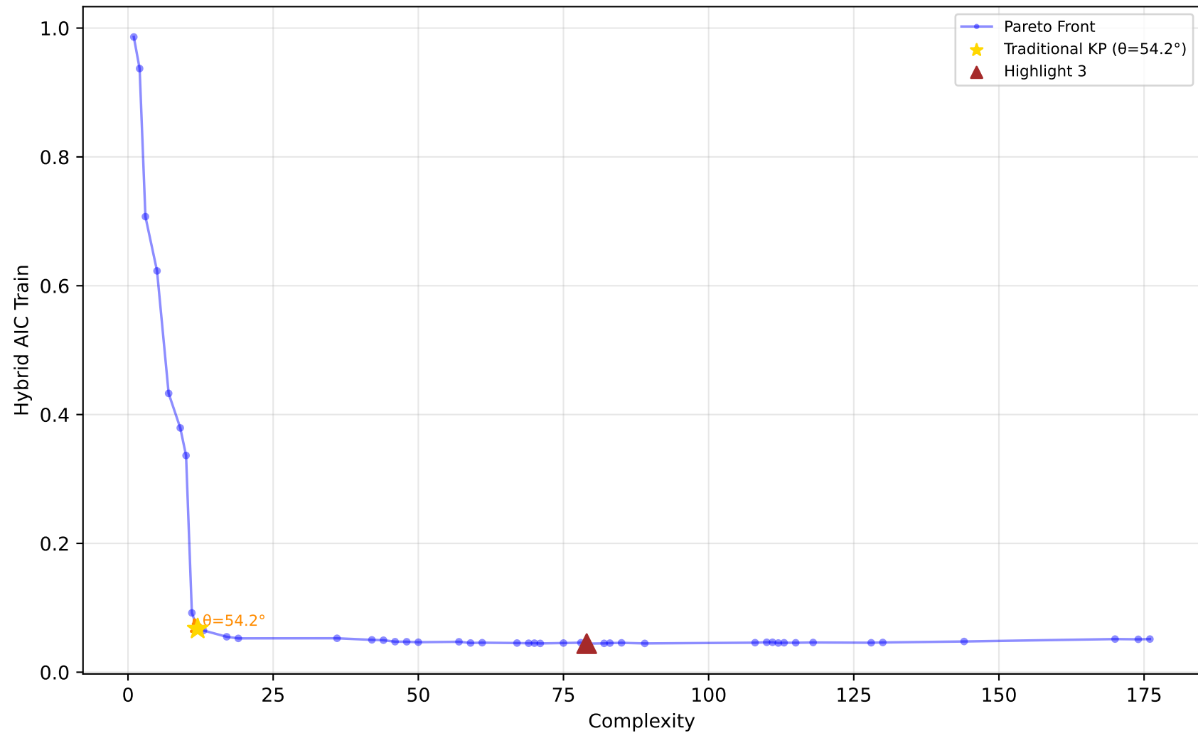
529_pollen - Run 1 - SVP - Hybrid AIC Train \lambda_1=0.10, \lambda_2=0.80, \lambda_3=0.30 | Difficulty: 1.00 | Method: hmr
