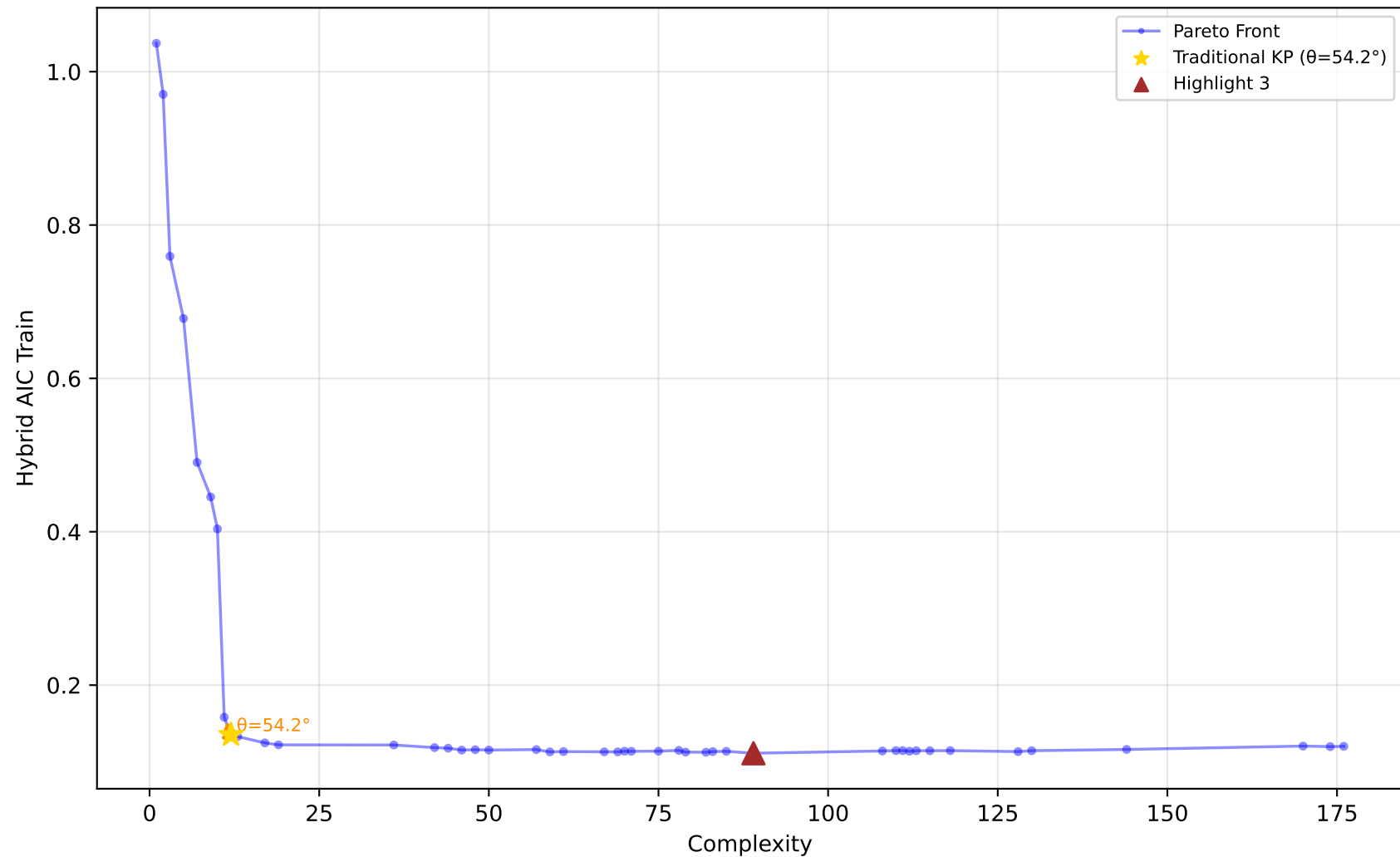
529_pollen - Run 1 - SVP - Hybrid AIC Train \lambda_1=0.60, \lambda_2=0.40, \lambda_3=1.00 | Difficulty: 1.00 | Method: hmr
