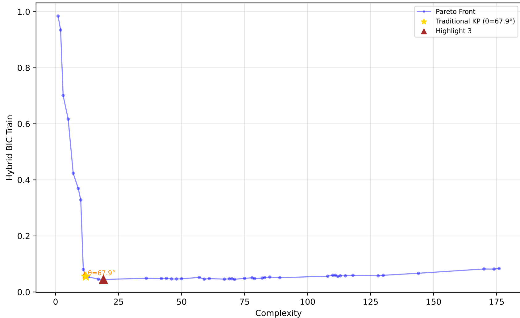
529_pollen - Run 1 - SVP - Hybrid BIC Train \lambda_1=0.10, \lambda_2=0.80, \lambda_3=0.30 | Difficulty: 1.00 | Method: hmr
