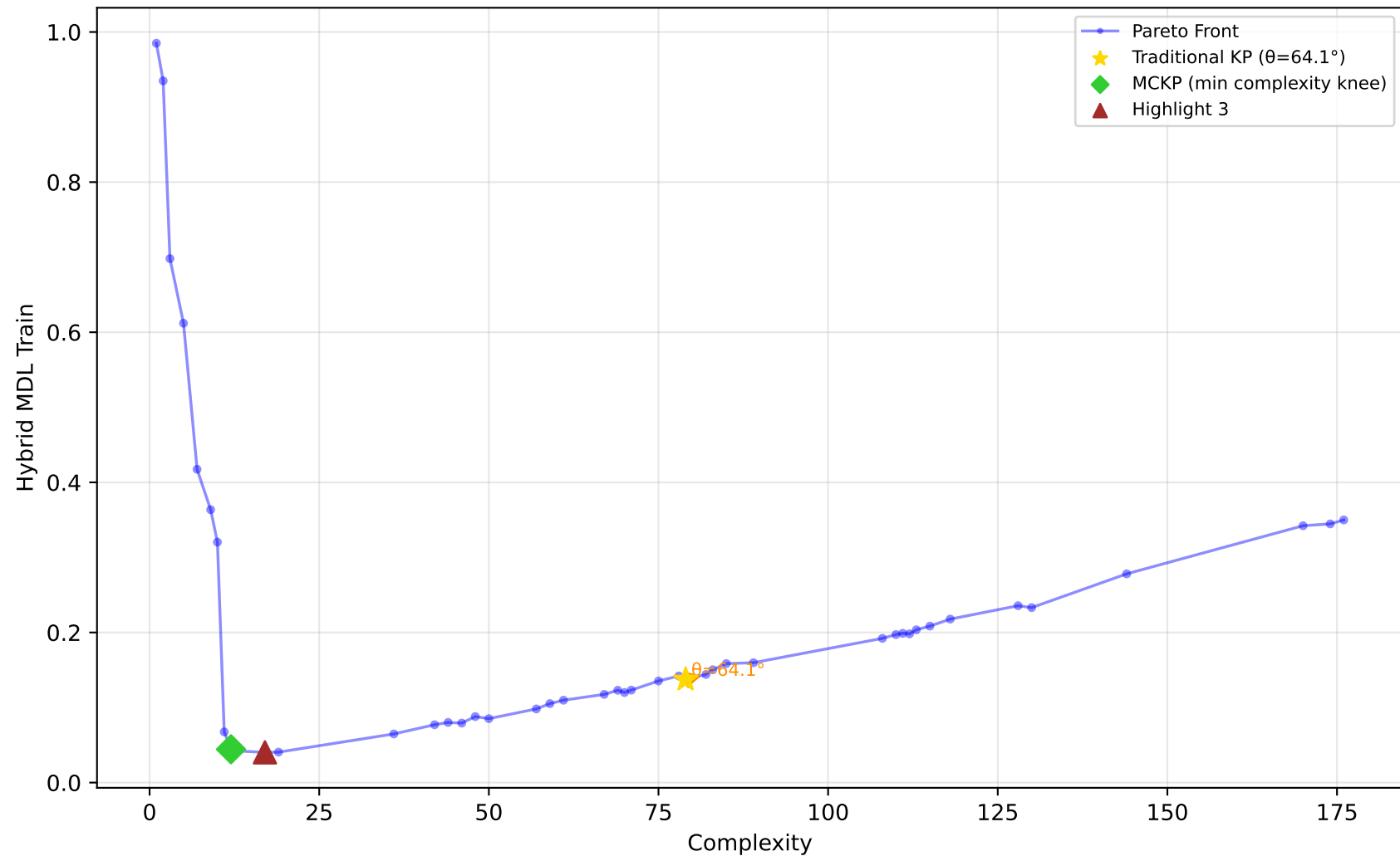
529_pollen - Run 1 - SVP - Hybrid MDL Train \lambda_1=0.10, \lambda_2=0.80, \lambda_3=0.30 | Difficulty: 1.00 | Method: hmr
