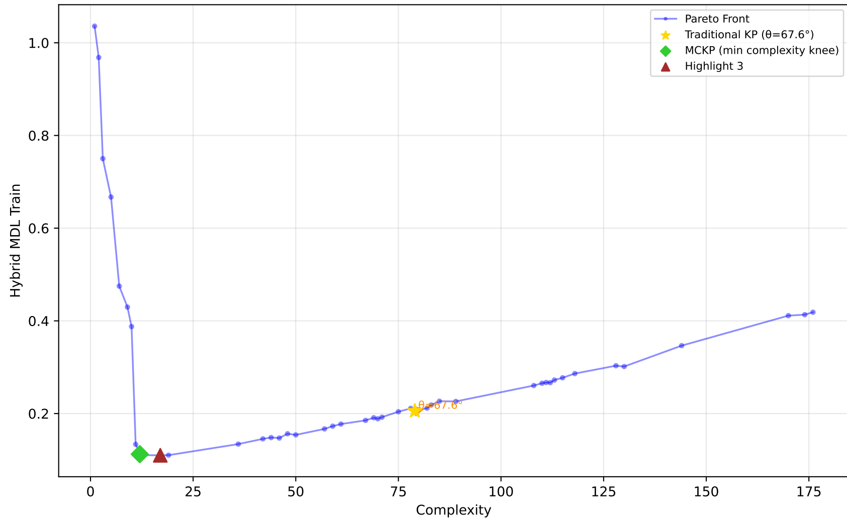
529_pollen - Run 1 - SVP - Hybrid MDL Train \lambda_1=0.60, \lambda_2=0.40, \lambda_3=1.00 | Difficulty: 1.00 | Method: hmr
