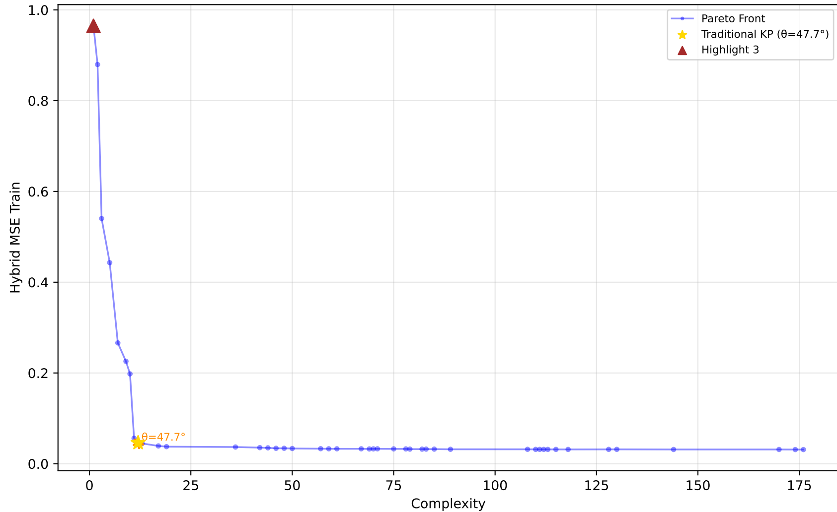
529_pollen - Run 1 - SVP - Hybrid MSE Train \lambda_1=0.10, \lambda_2=0.80, \lambda_3=0.30 | Difficulty: 1.00 | Method: hmr
