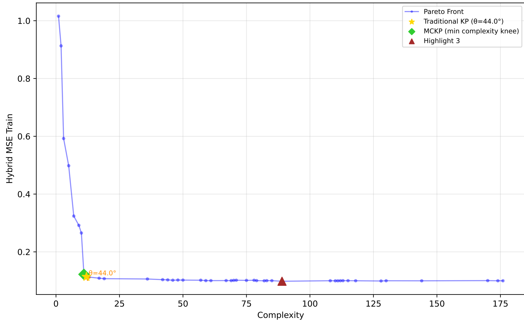
529_pollen - Run 1 - SVP - Hybrid MSE Train \lambda_1=0.60, \lambda_2=0.40, \lambda_3=1.00 | Difficulty: 1.00 | Method: hmr
