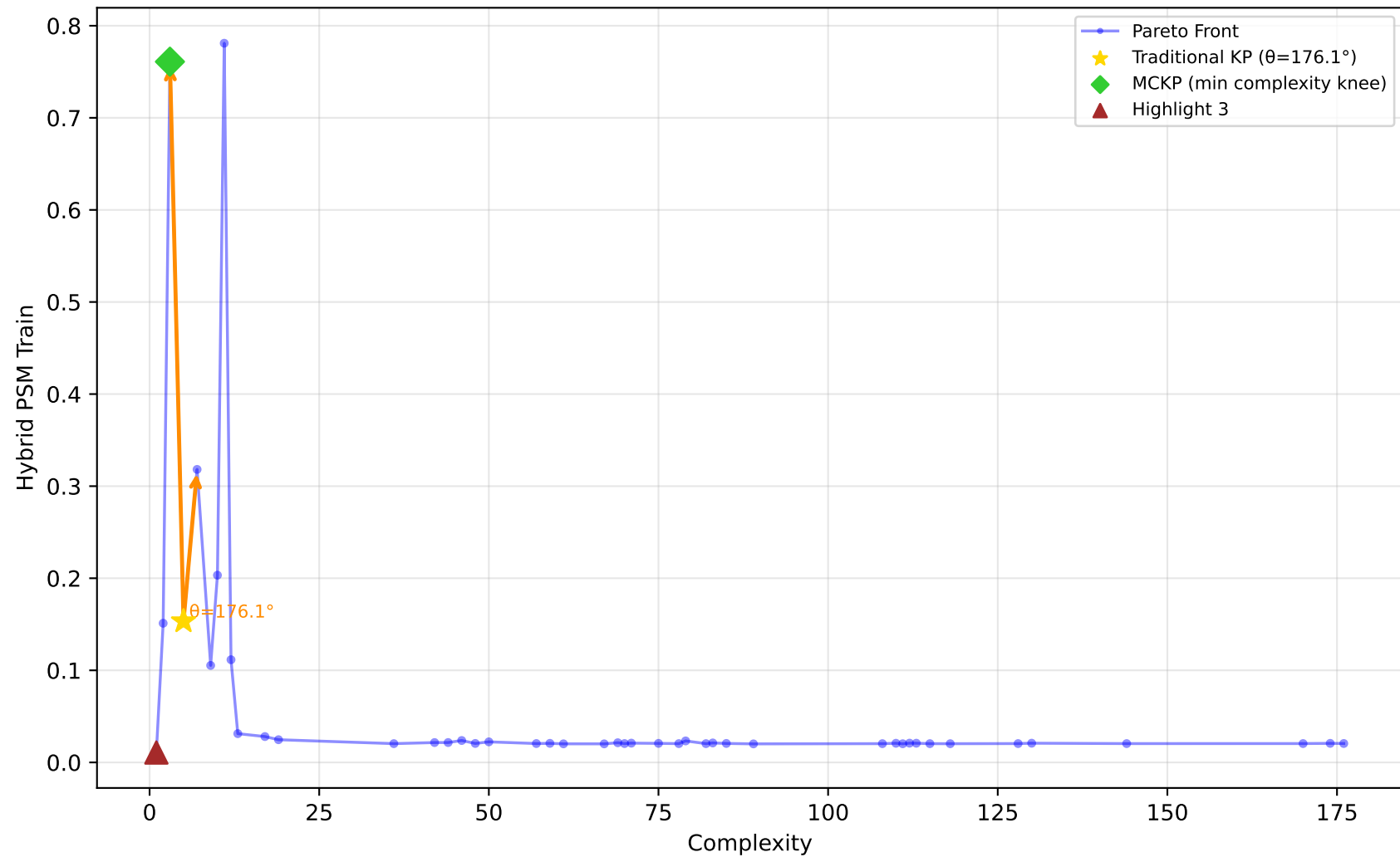
529_pollen - Run 1 - SVP - Hybrid PSM Train \lambda_1=0.10, \lambda_2=0.80, \lambda_3=0.30 | Difficulty: 1.00 | Method: hmr
