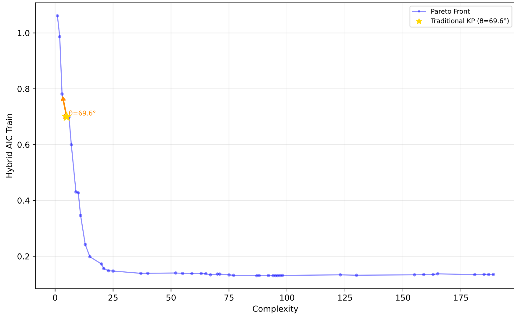
529_pollen - Run 20 - MVP - Hybrid AIC Train \lambda_1=0.90, \lambda_2=0.00, \lambda_3=0.00 | Difficulty: 1.00 | Method: hmr
