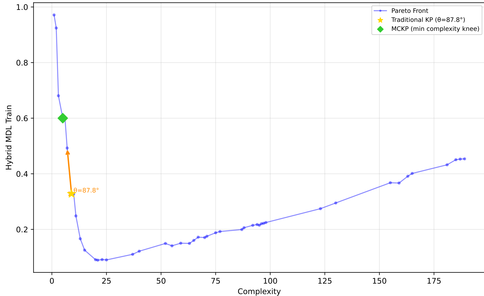
529_pollen - Run 20 - MVP - Hybrid MDL Train \lambda_1=0.00, \lambda_2=1.00, \lambda_3=0.80 | Difficulty: 1.00 | Method: hmr
