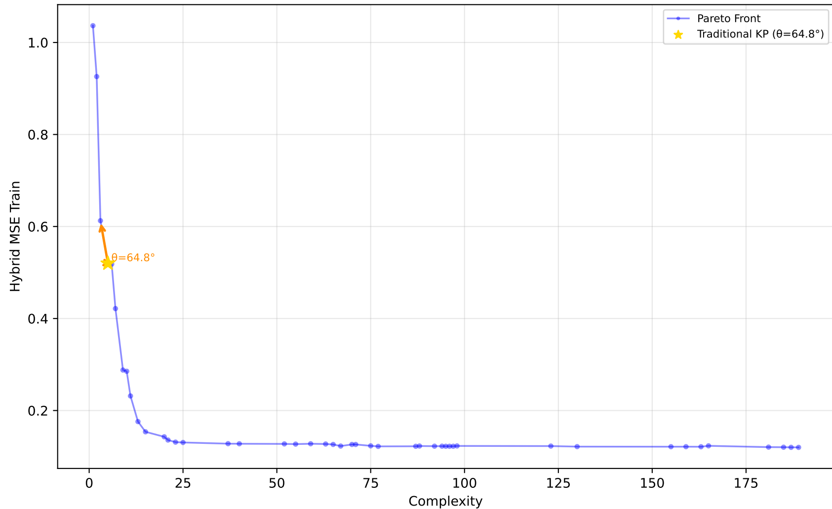
529_pollen - Run 20 - MVP - Hybrid MSE Train \lambda_1=0.90, \lambda_2=0.00, \lambda_3=0.00 | Difficulty: 1.00 | Method: hmr
