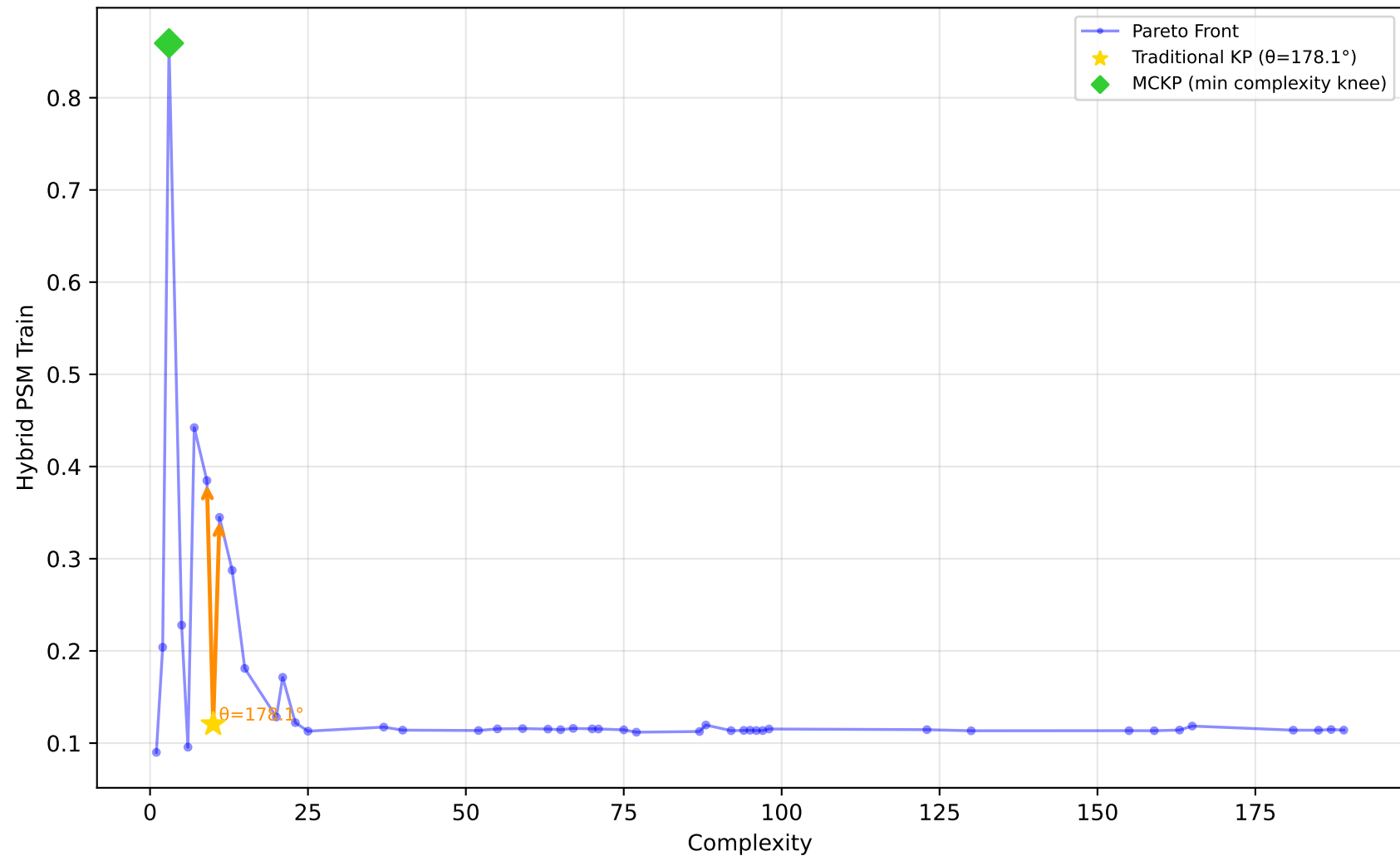
529_pollen - Run 20 - MVP - Hybrid PSM Train \lambda_1=0.90, \lambda_2=0.00, \lambda_3=0.00 | Difficulty: 1.00 | Method: hmr
