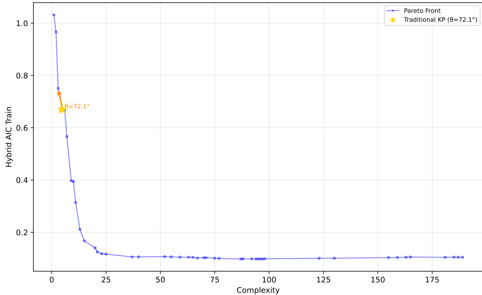
529_pollen - Run 20 - SVP - Hybrid AIC Train \lambda_1=0.60, \lambda_2=0.40, \lambda_3=1.00 | Difficulty: 1.00 | Method: hmr
