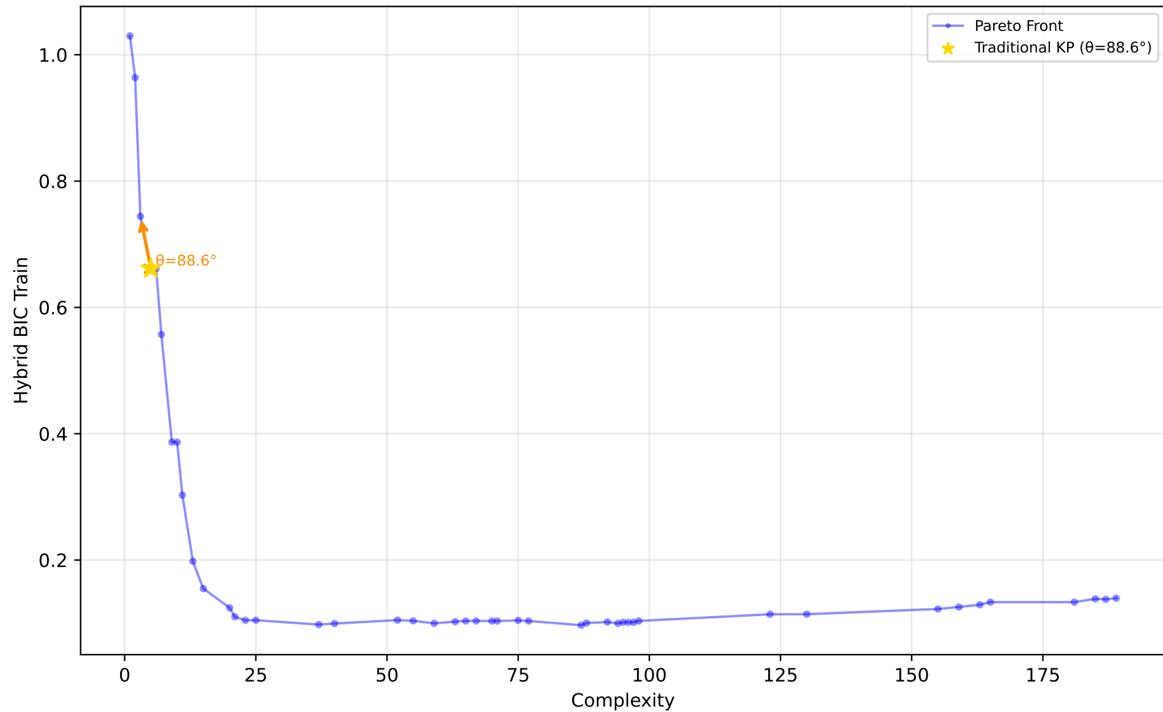
529_pollen - Run 20 - SVP - Hybrid BIC Train \lambda_1=0.60, \lambda_2=0.40, \lambda_3=1.00 | Difficulty: 1.00 | Method: hmr
