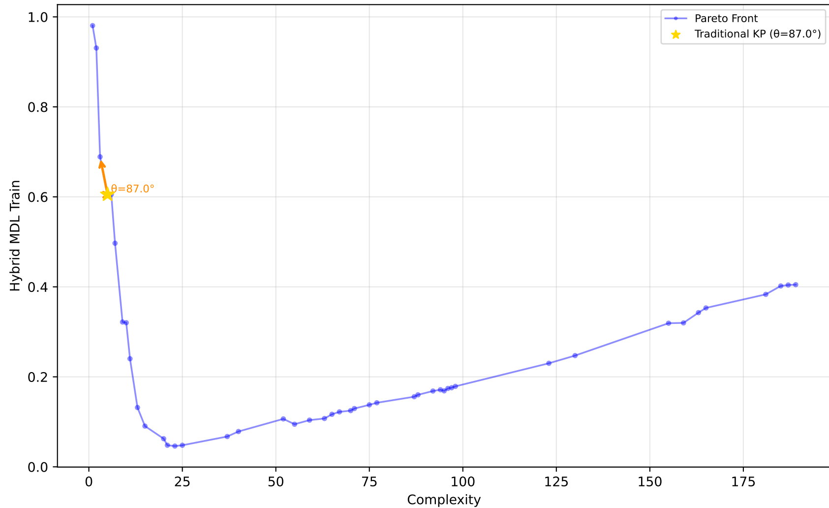
529_pollen - Run 20 - SVP - Hybrid MDL Train \lambda_1=0.10 , \lambda_2=0.80 , \lambda_3=0.30 | Difficulty: 1.00 | Method: hmr
