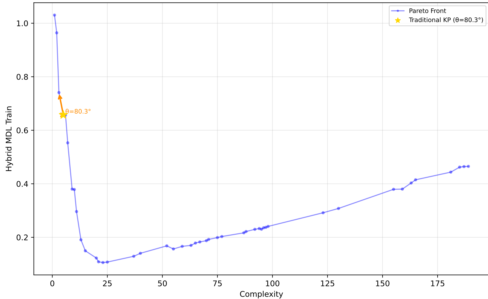
529_pollen - Run 20 - SVP - Hybrid MDL Train \lambda_1=0.60, \lambda_2=0.40, \lambda_3=1.00 | Difficulty: 1.00 | Method: hmr
