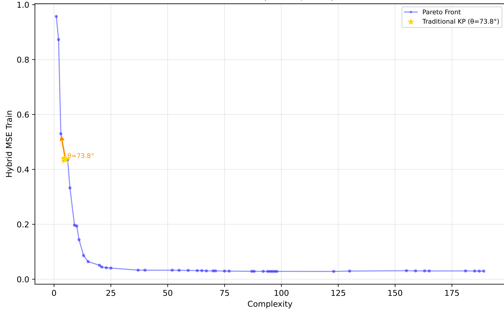
529_pollen - Run 20 - SVP - Hybrid MSE Train \lambda_1=0.10, \lambda_2=0.80, \lambda_3=0.30 | Difficulty: 1.00 | Method: hmr
