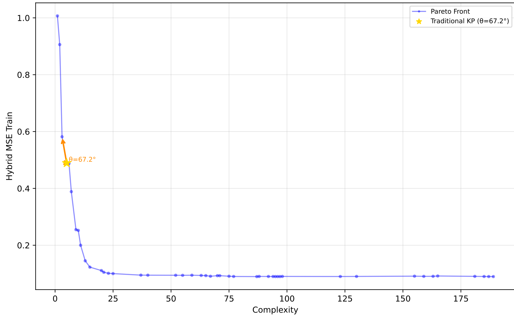
529_pollen - Run 20 - SVP - Hybrid MSE Train \lambda_1=0.60, \lambda_2=0.40, \lambda_3=1.00 | Difficulty: 1.00 | Method: hmr
