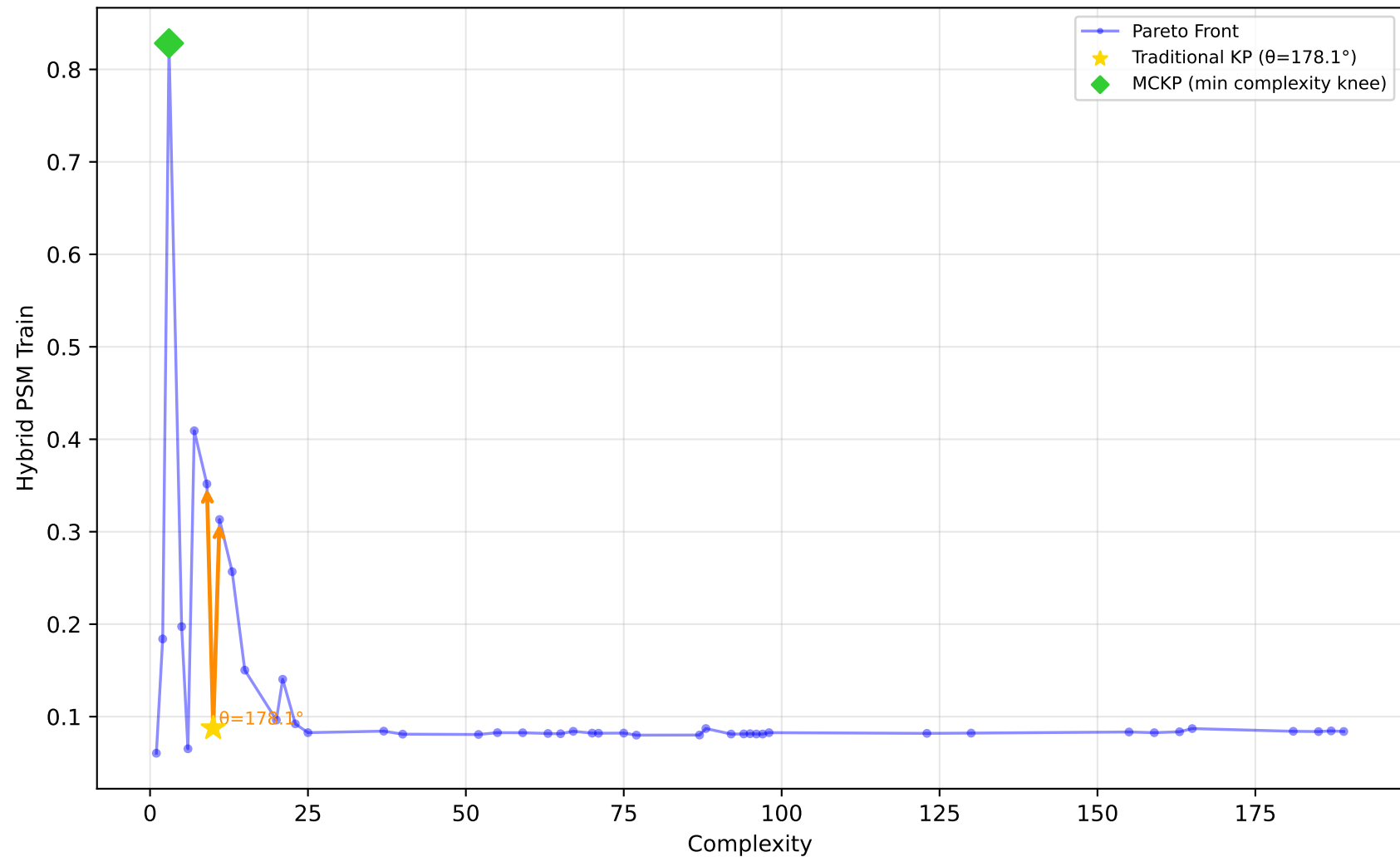
529_pollen - Run 20 - SVP - Hybrid PSM Train \lambda_1=0.60, \lambda_2=0.40, \lambda_3=1.00 | Difficulty: 1.00 | Method: hmr
