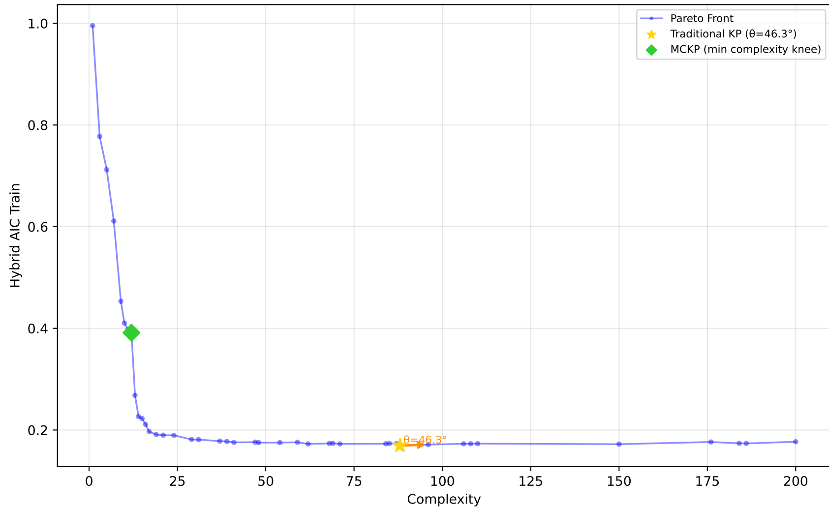
529_pollen - Run 21 - MVP - Hybrid AIC Train \lambda_1=0.90, \lambda_2=0.00, \lambda_3=0.00 | Difficulty: 1.00 | Method: hmr
