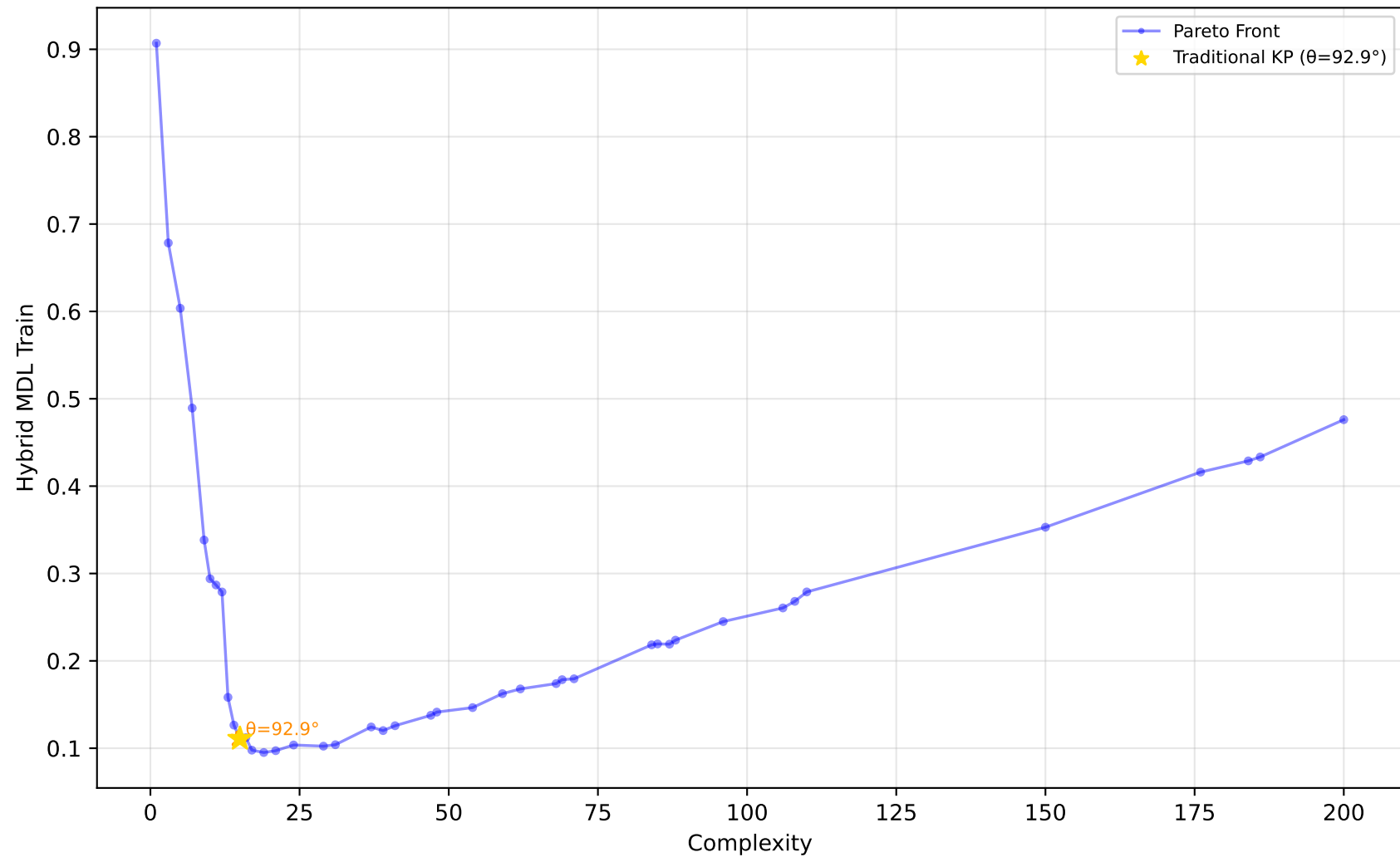
529_pollen - Run 21 - MVP - Hybrid MDL Train \lambda_1=0.00, \lambda_2=1.00, \lambda_3=0.80 | Difficulty: 1.00 | Method: hmr
