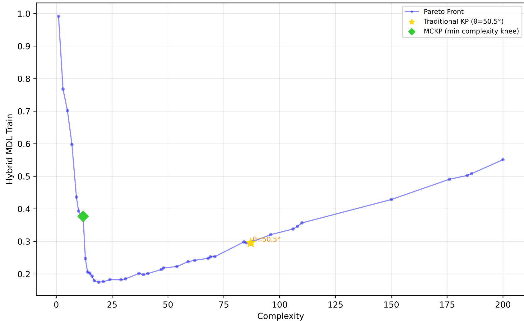
529_pollen - Run 21 - MVP - Hybrid MDL Train \lambda_1=0.90, \lambda_2=0.00, \lambda_3=0.00 | Difficulty: 1.00 | Method: hmr
