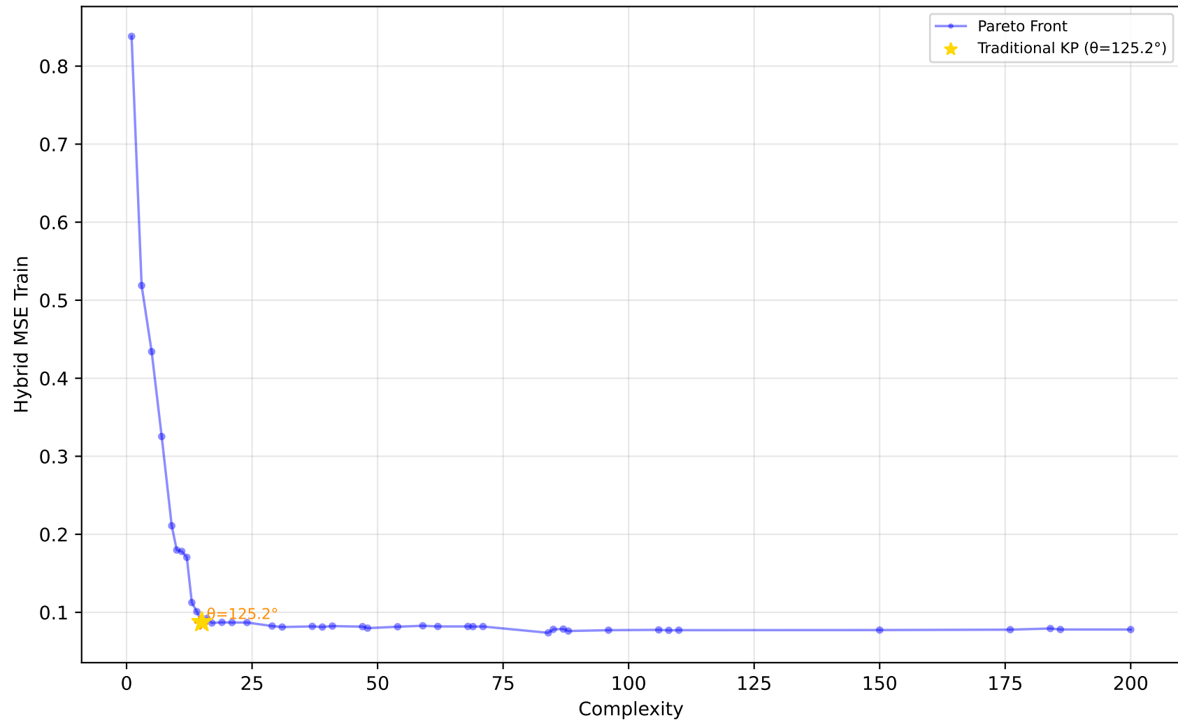
529_pollen - Run 21 - MVP - Hybrid MSE Train \lambda_1=0.00, \lambda_2=1.00, \lambda_3=0.80 | Difficulty: 1.00 | Method: hmr
