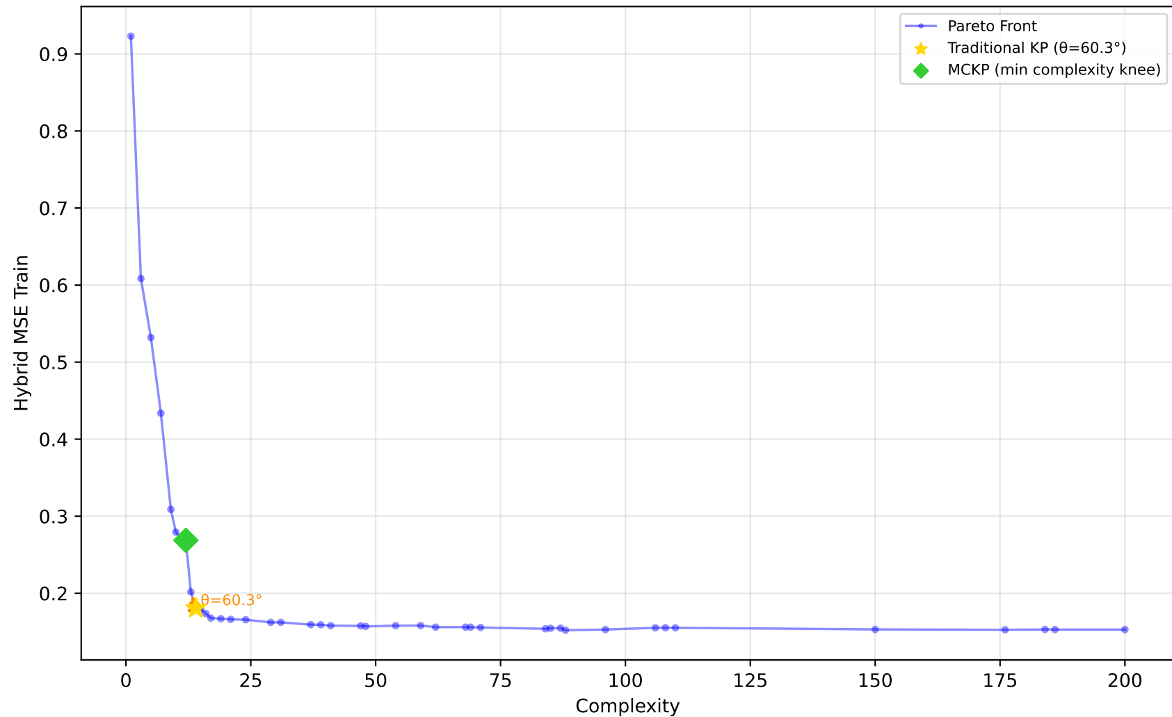
529_pollen - Run 21 - MVP - Hybrid MSE Train \lambda_1=0.90, \lambda_2=0.00, \lambda_3=0.00 | Difficulty: 1.00 | Method: hmr
