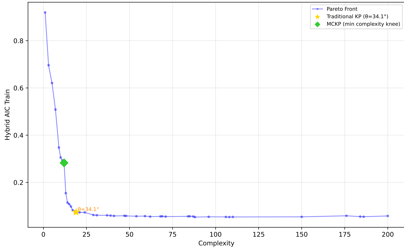
529_pollen - Run 21 - SVP - Hybrid AIC Train \lambda_1=0.10 , \lambda_2=0.80 , \lambda_3=0.30 | Difficulty: 1.00 | Method: hmr
