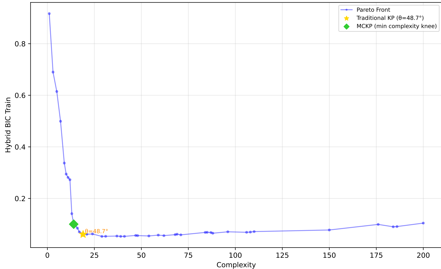
529_pollen - Run 21 - SVP - Hybrid BIC Train \lambda_1=0.10 , \lambda_2=0.80 , \lambda_3=0.30 | Difficulty: 1.00 | Method: hmr
