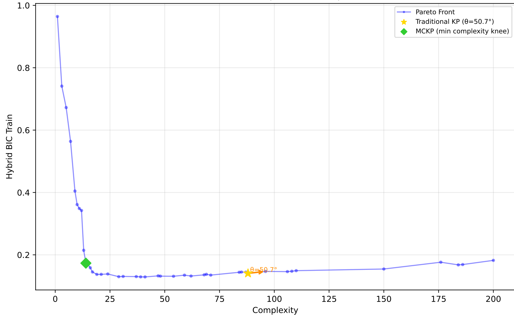
529_pollen - Run 21 - SVP - Hybrid BIC Train \lambda_1=0.60, \lambda_2=0.40, \lambda_3=1.00 | Difficulty: 1.00 | Method: hmr
